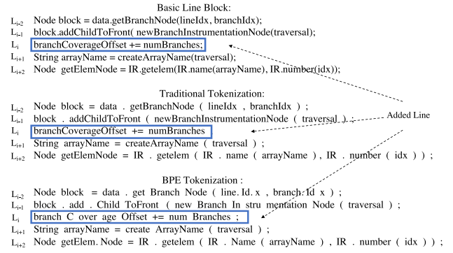
Fig. 5. Tokenize example.
